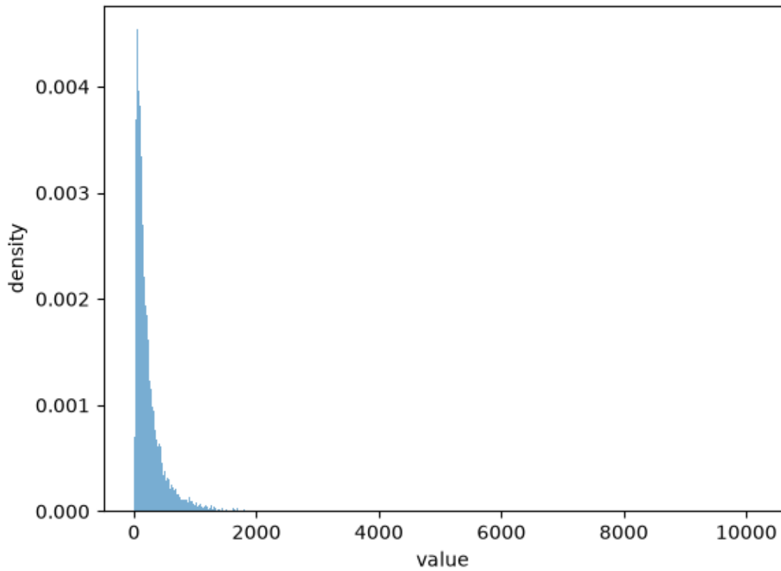
Fig. 14.1: Sample histogram of one lognormal
