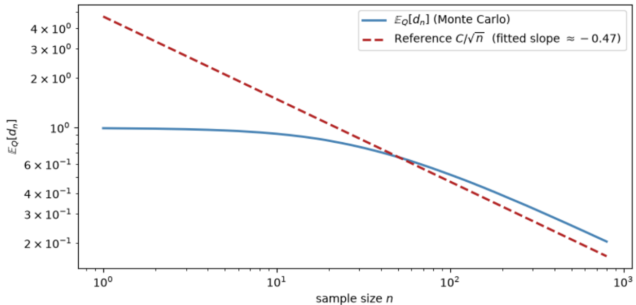
Fig. 34.8: A log-log plot of the average merging distance in the Beta-Bernoulli model. The fitted slope is close to -1/2 , which is consistent with square-root decay in this experiment.
