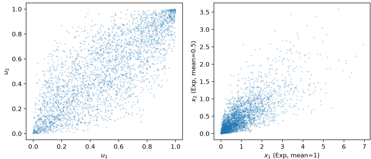
Fig. 8.1: gaussian copula with exponential marginals
