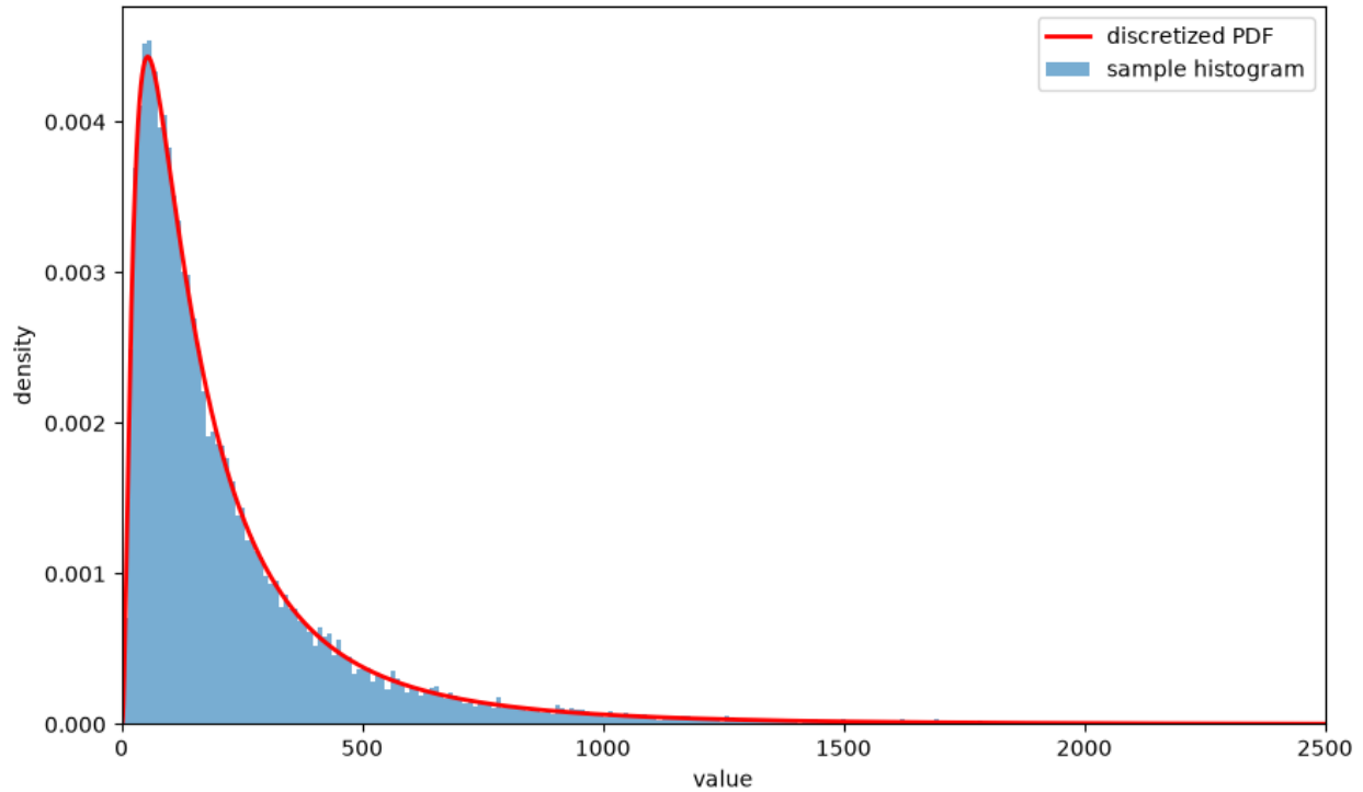
Fig. 14.4: Discretized density against sample
