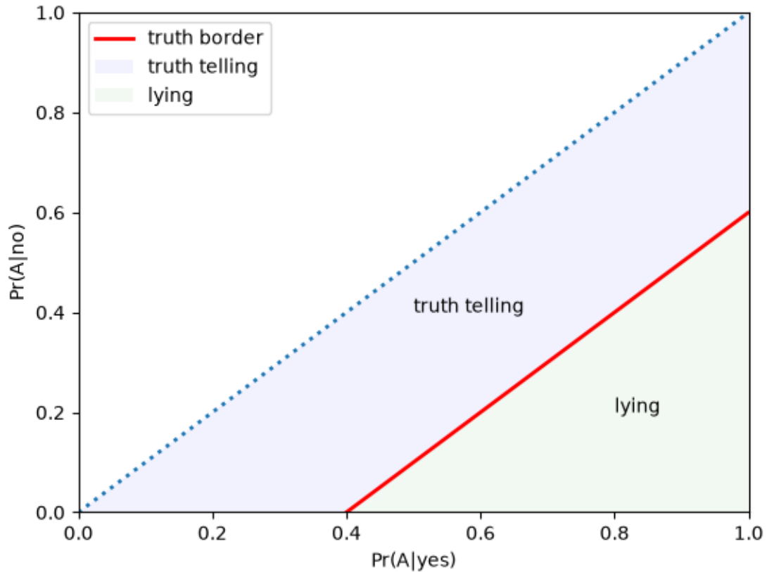
Fig. 17.2: Truth telling and lying areas
