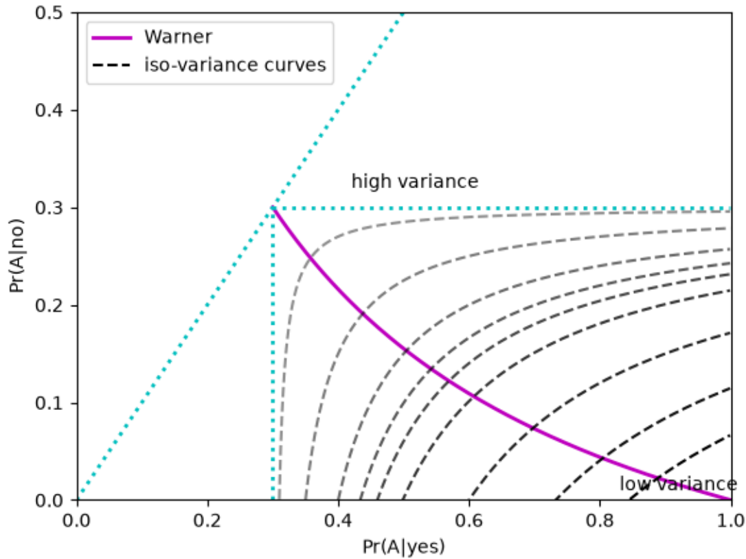
Fig. 17.3: Iso-variance curves
