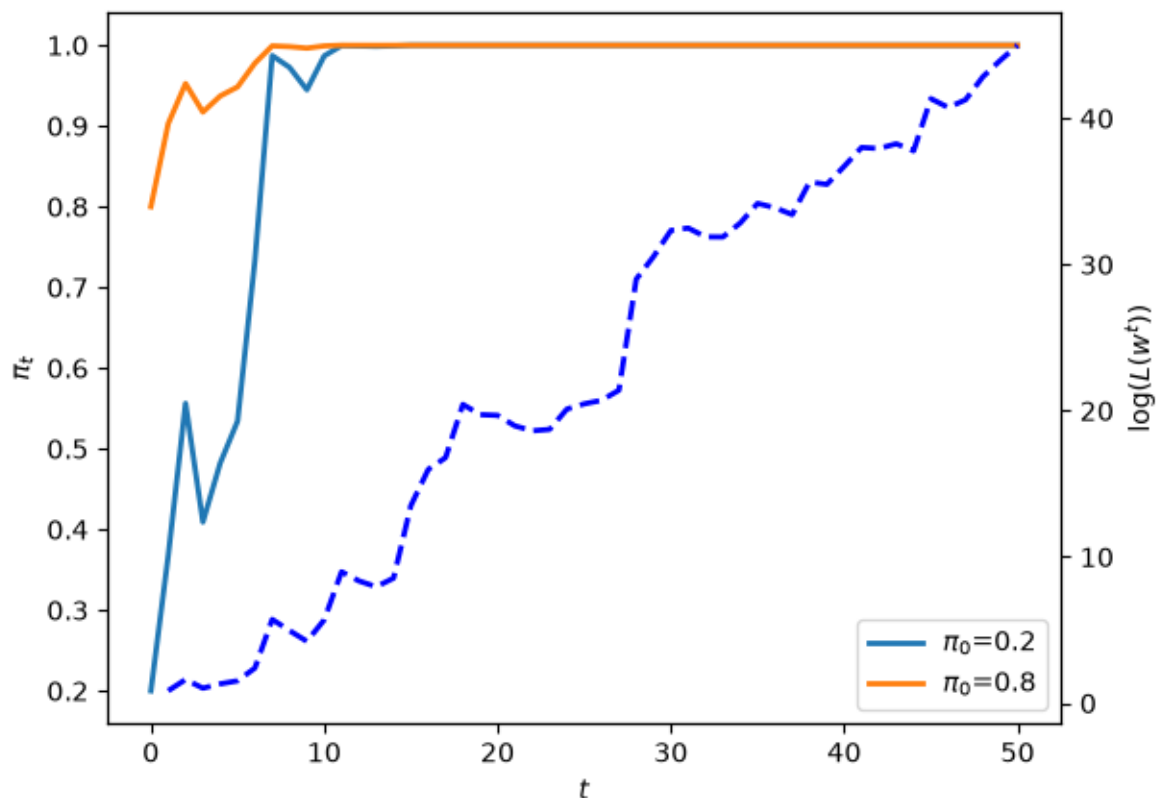
Fig. 29.1: Posterior paths and log likelihood
