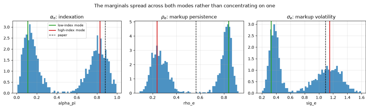
Fig. 139.1: Marginal posteriors for the parameters that separate the two modes
