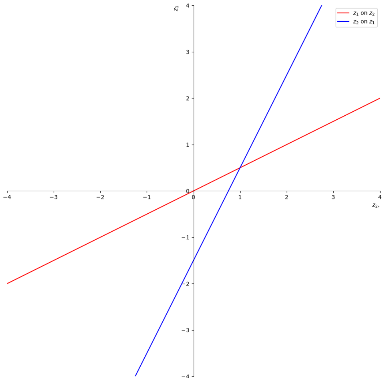
Fig. 13.1: two regressions
