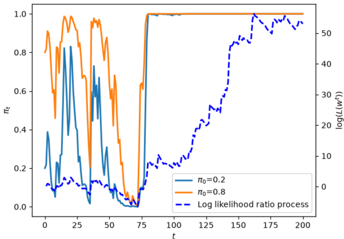
Fig. 32.2: Belief paths, \alpha = 0.6
