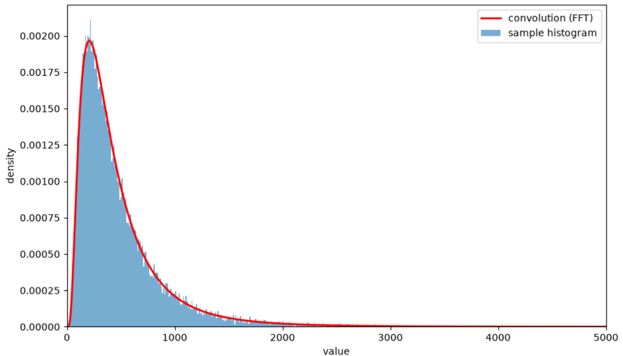
Fig. 14.5: Convolution against sample, two components
