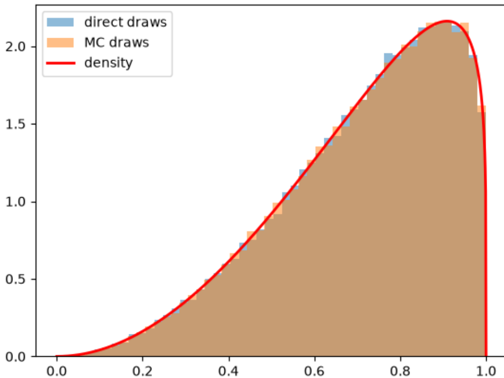
Fig. 32.1: Direct and Monte Carlo draws
